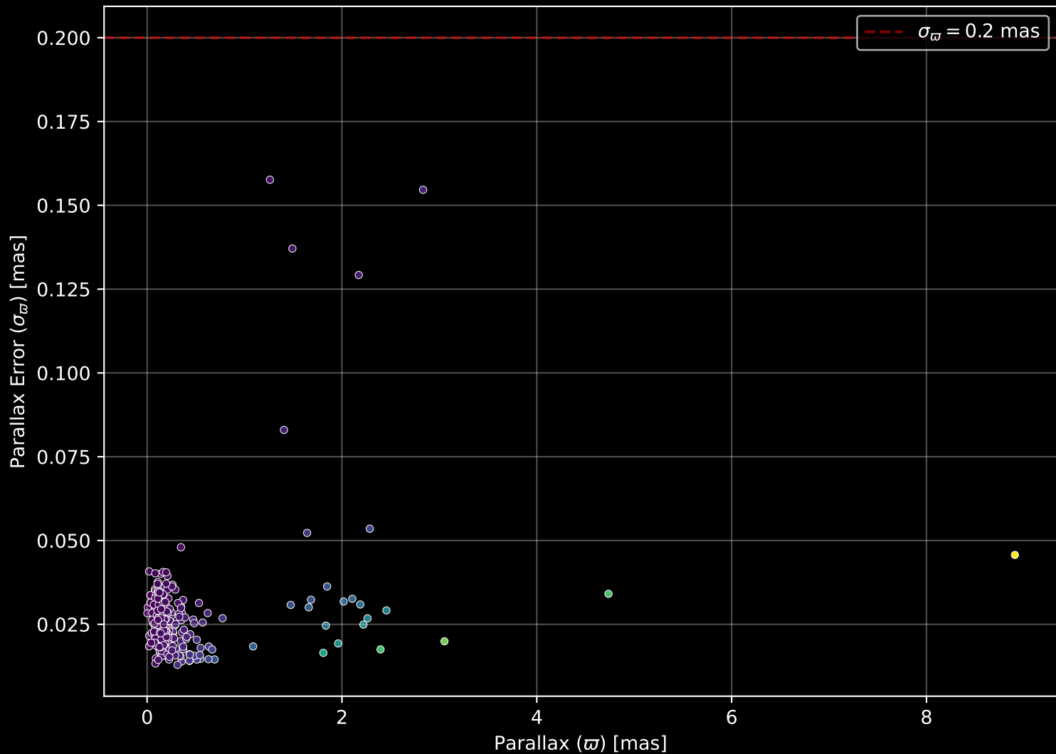
APOGEE DR17 Field: [020-12] Parallax Quality (n= 273)
