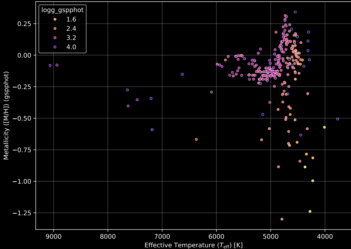
APOGEE DR17 Field: [020-12] Stellar Population Parameters (n= 273)
