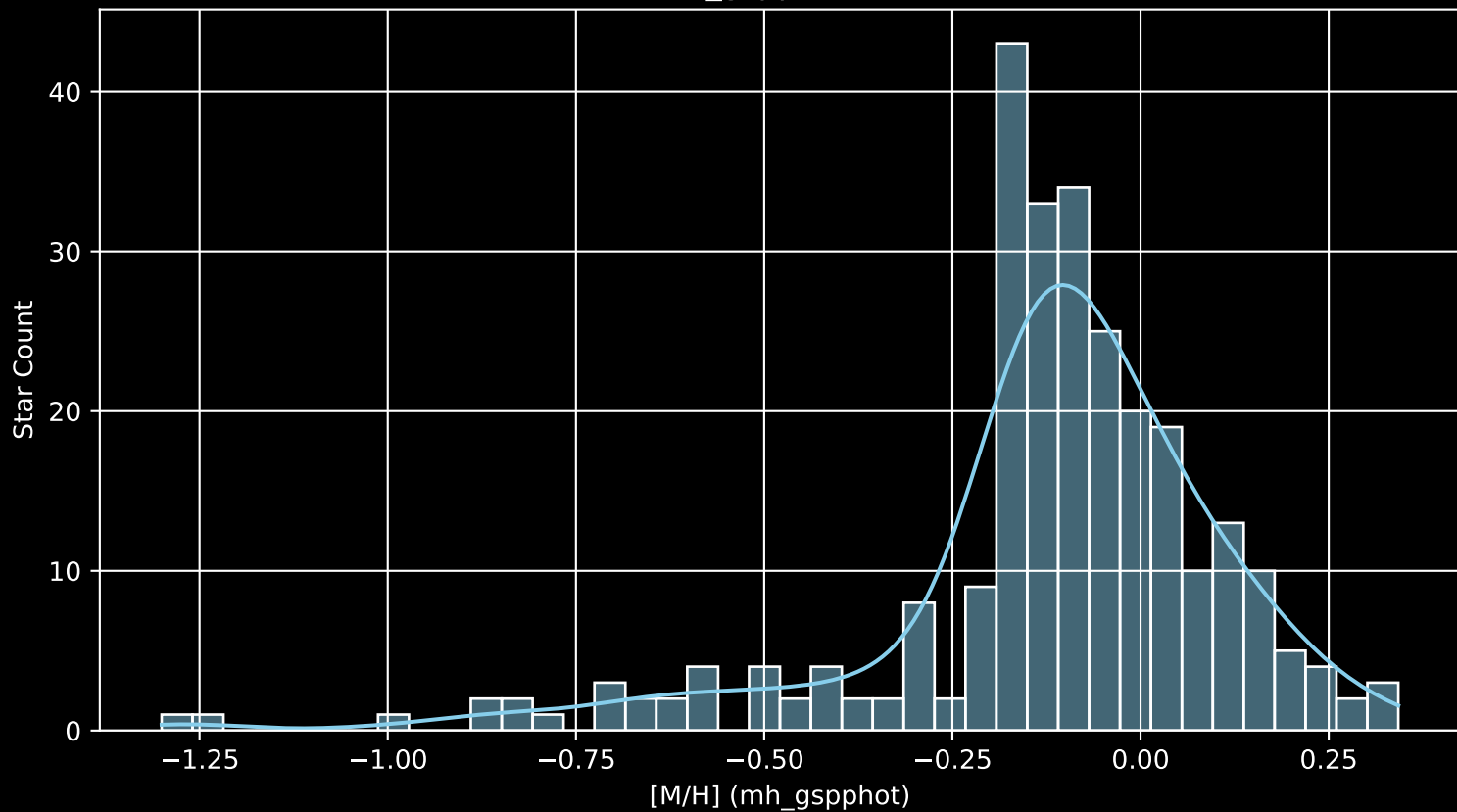
APOGEE DR17 Field: [020-12 [M/H] (mh_gspphot) (n= 273)
