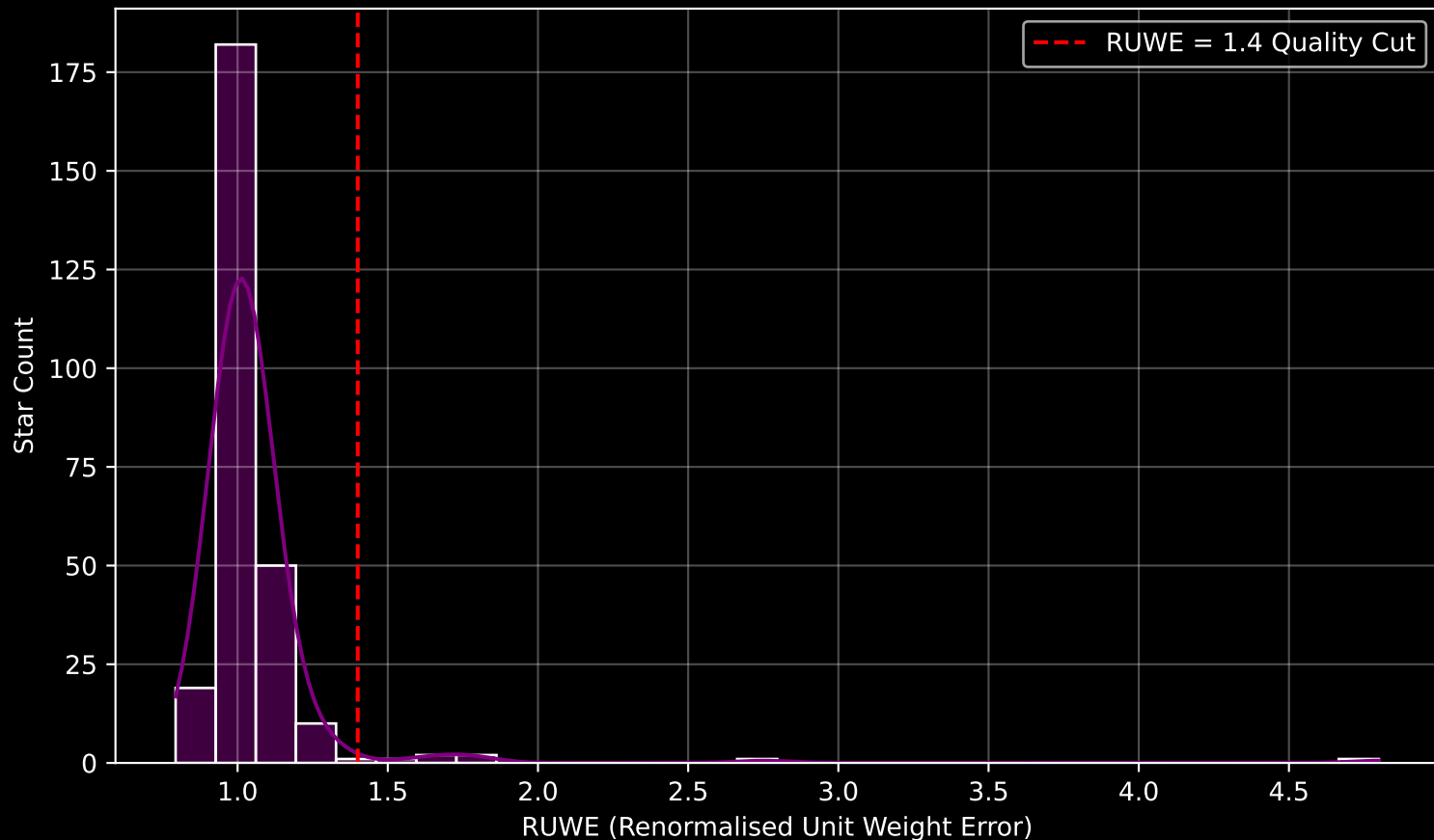
GAPOGEE DR17 Field [020-12] RUWE Distribution (n= 269)
