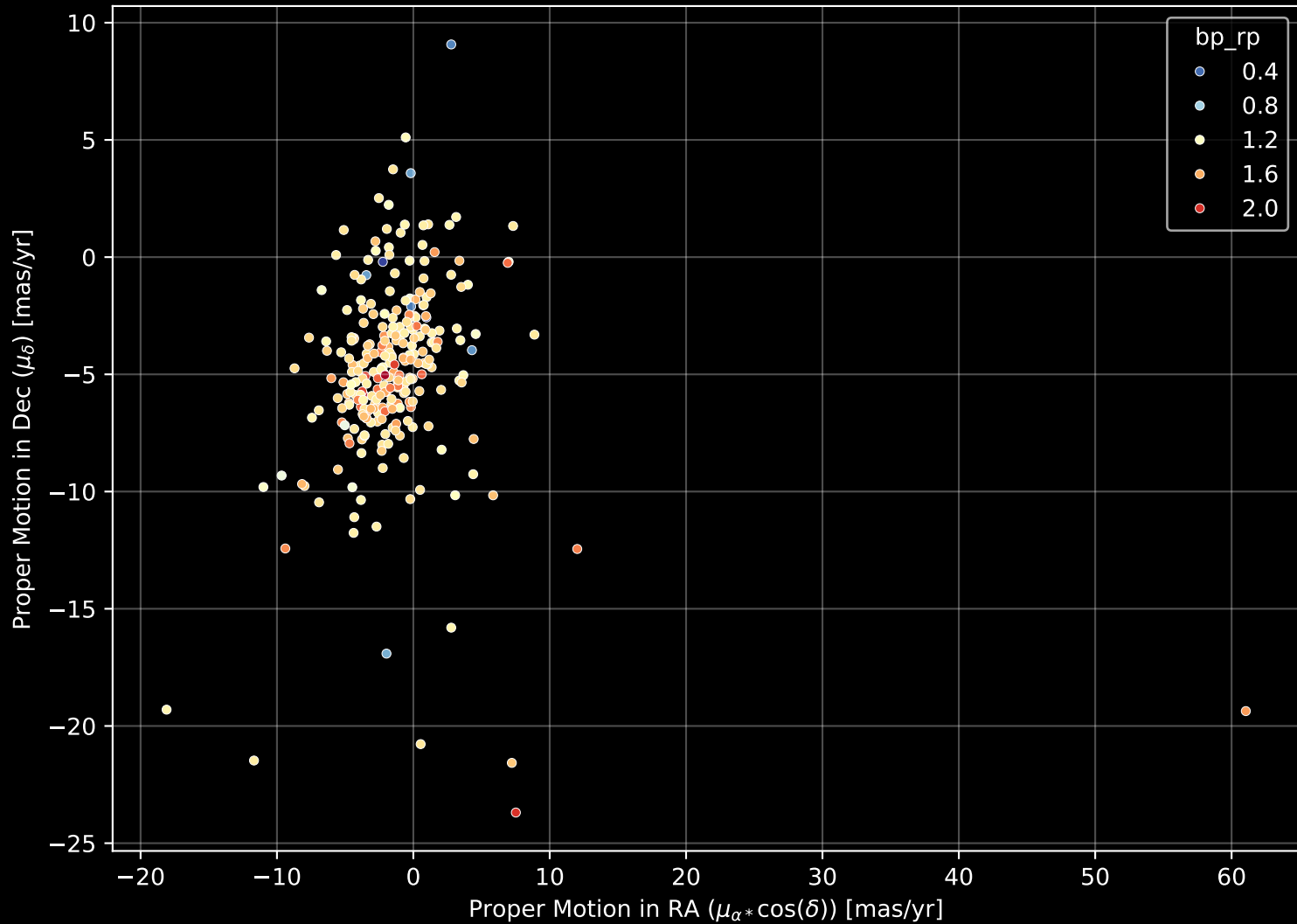
APOGEE DR17 Field: [020-12] Proper Motion Diagram (n= 273)
