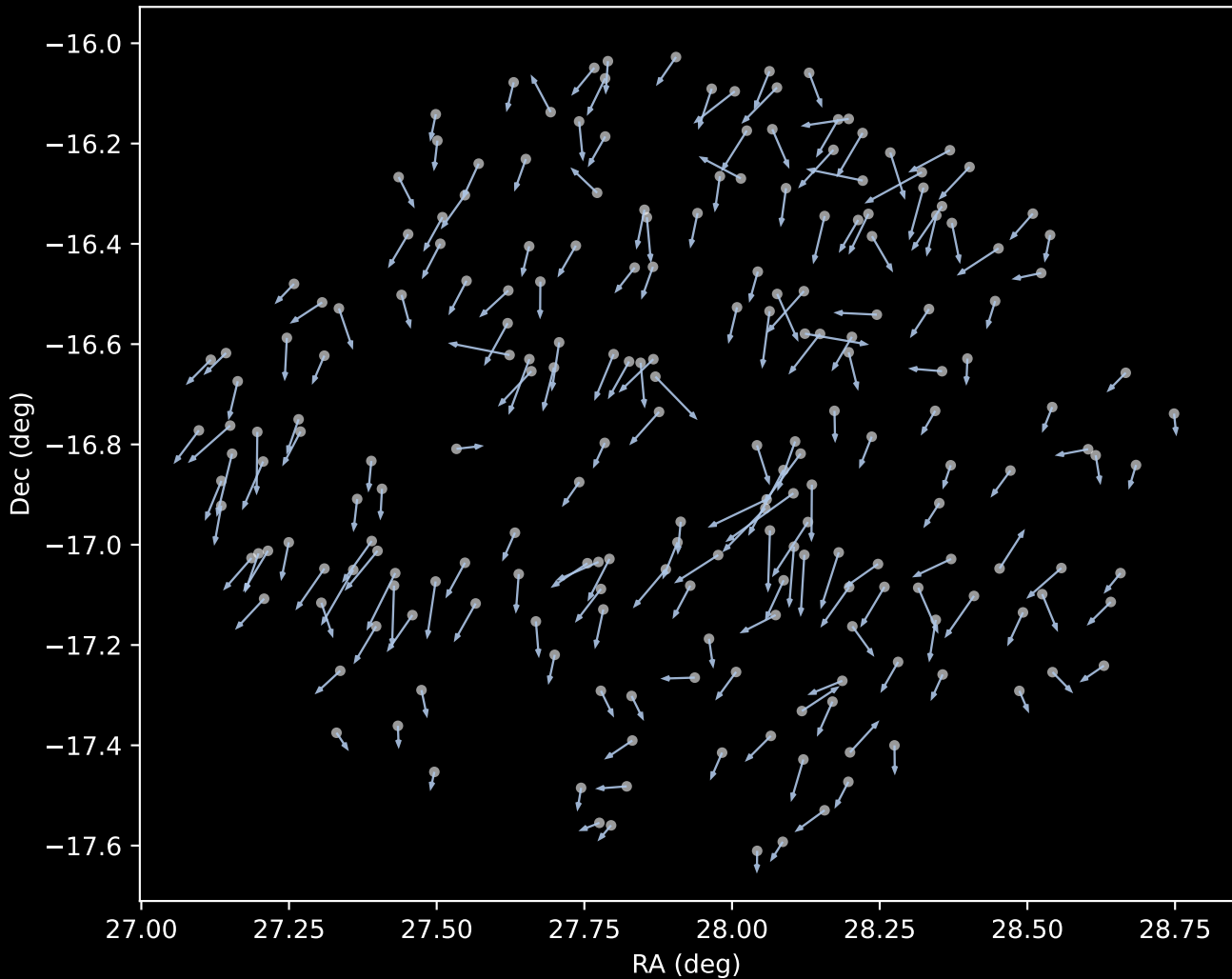
APOGEE DR17 Cluster 1 Proper Motion Vectors (n=213)
